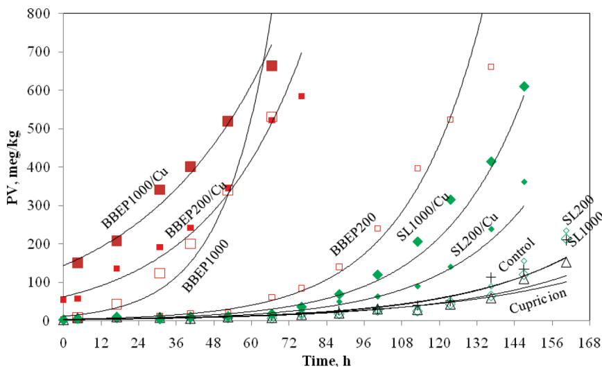
Figure 1. PV development of purified soybean oil at 32 °C in the presence of SL and BBEP fractions (200 and 1000 ppm) and cupric ion (8 ppm). Trend lines are drawn by following exponential regression models. For treatment abbreviations, refer to the footnotes of Tables 1 and 2 .
