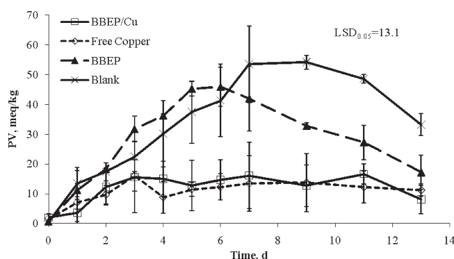
Figure 3. PV development of egg phospholipids in liposome at 60 °C in the presence of BBEP (1000 ppm) and cupric ion (8 ppm). Error bars represent SD from duplicate preparations. For treatment abbreviations, refer to the footnotes of Tables 1 and 2 .
