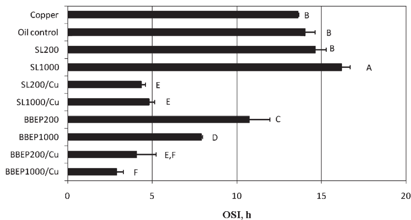
Figure 2. OSI value (time, h) of commercial soybean oil (CSO) at 100 °C in the presence of SL and BBEP fraction (200 and 1000 ppm) and cupric ion (8 ppm). Error bars represent SD from duplicate preparations. For treatment abbreviations, refer to the footnotes of Tables 1 and 2 . Different letters represent the least significant difference at P < 0.05 .
